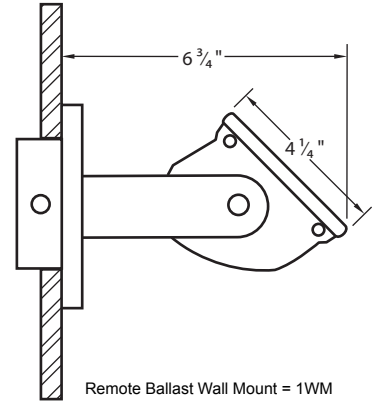
Remote Ballast Wall Mount = 1WM
