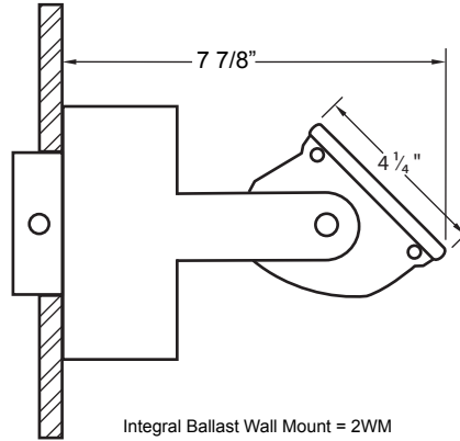
Integral Ballast Wall Mount = 2WM
