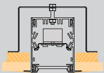
Recessed Mount: Mud In (FF)
