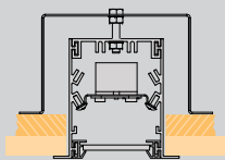
Recessed Mount: Flanged (F)
