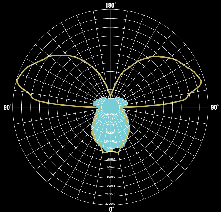
CANDELA PLOT — 0°-180° 90°-270°
